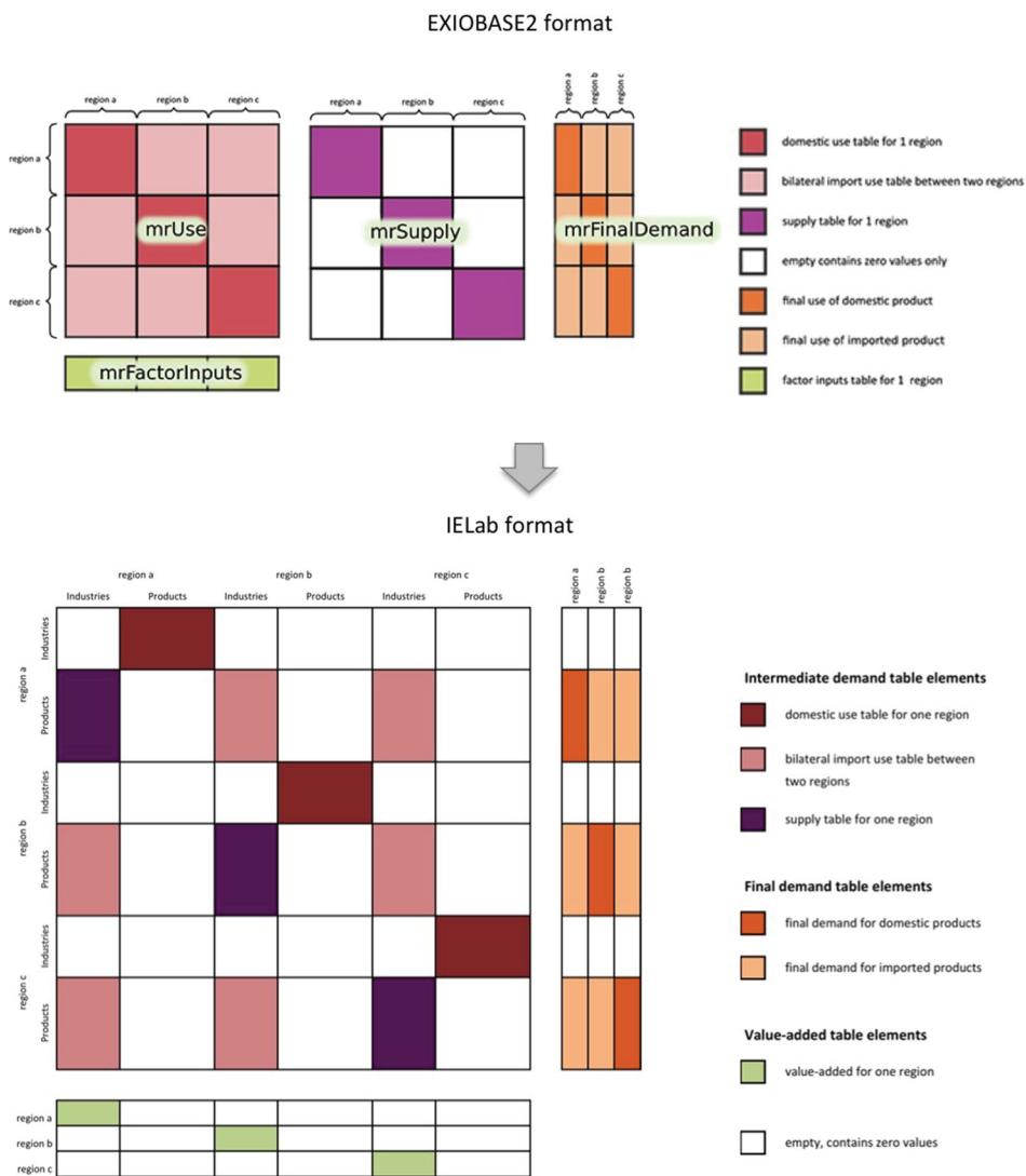
Figure 1. Schematic of the IELab MRIO format based on EXIOBASE2.
