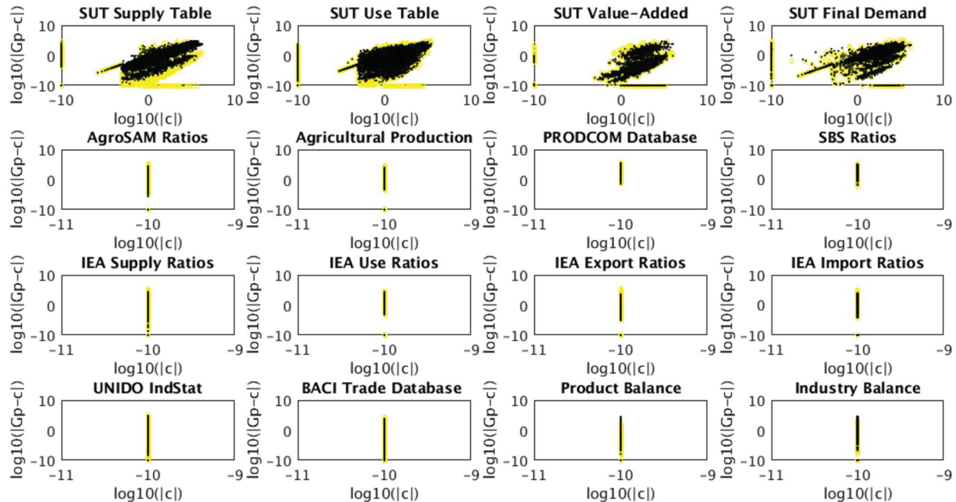
Figure 3. Detailed constraint violations in EXIOBASE2 (light) and IELab (dark), as implemented in the MRIO Lab.
