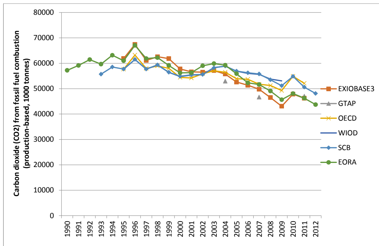
Figure 2: Production-based carbon footprint for Sweden (carbon dioxide emissions from fossil fuel combustion), 1990–2012, EXIOBASE3, GTAP, OECD, WIOD, SCB and Eora.
