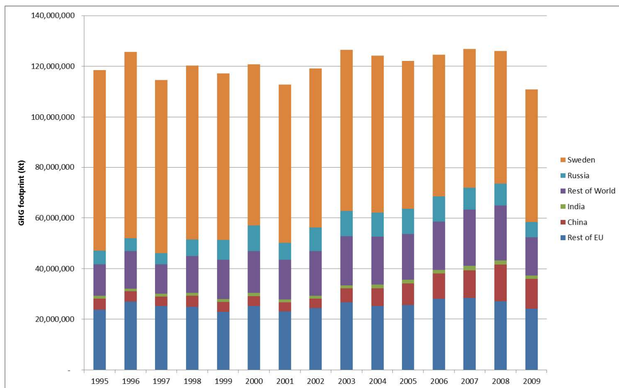
Figure 8: Change in top 6 hotspots of Sweden's GHG footprint, WIOD model 1995–2011
